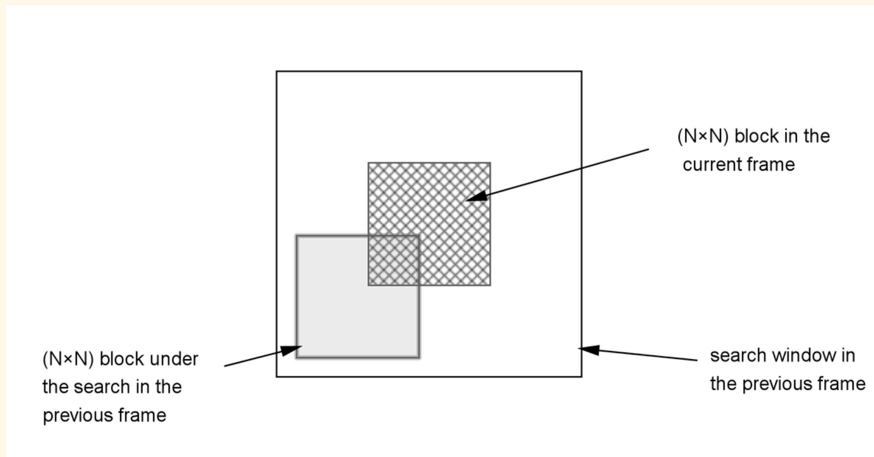
Alogithme de block matching [3]
